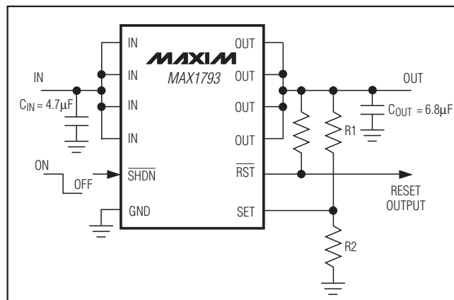
Figure 3. Typical Operating Circuit with Adjustable Output Voltage
