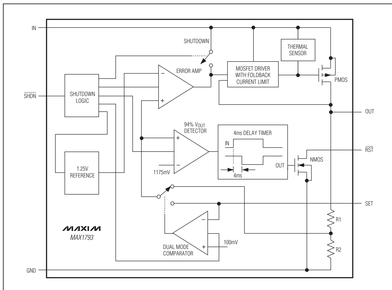
Figure 1. Functional Diagram
