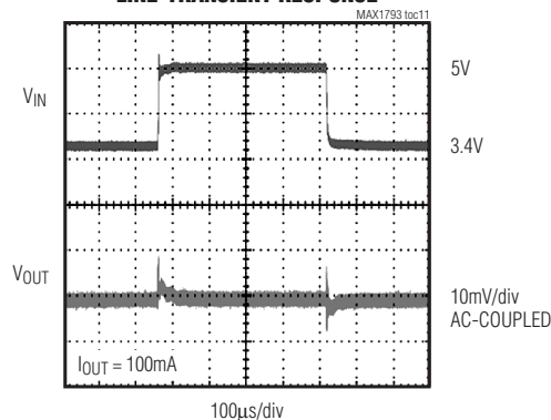
LINE-TRANSIENT RESPONSE
