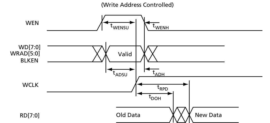
Figure 1-30 • 42MX SRAM Asynchronous Read Operation—Type 2
