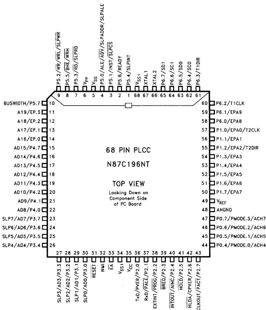
Figure 3. 68-Pin PLCC Package Diagram
