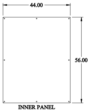
INNER PANEL
