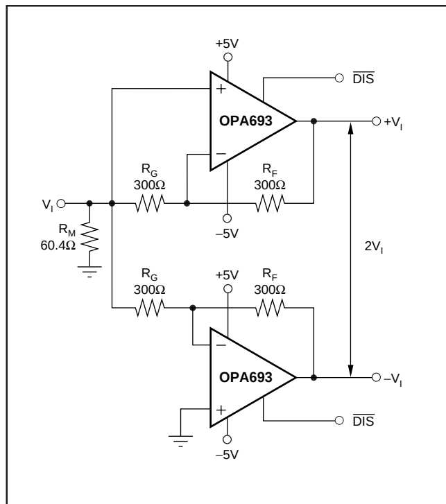
Figure 9. DC → 700MHz, Single-to-Differential Conversion.
