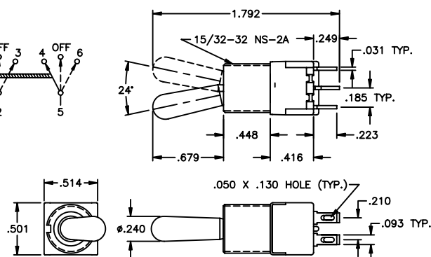
DOUBLE POLE
