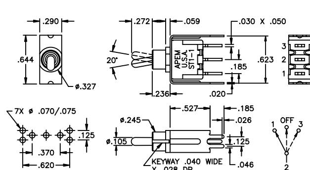
SINGLE POLE
