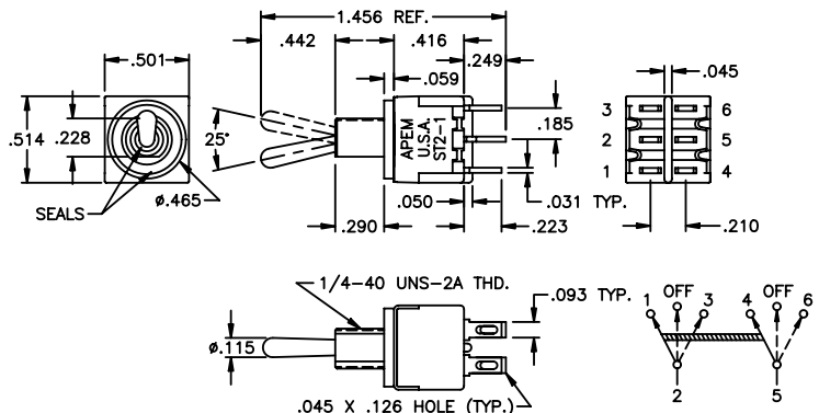
DOUBLE POLE
