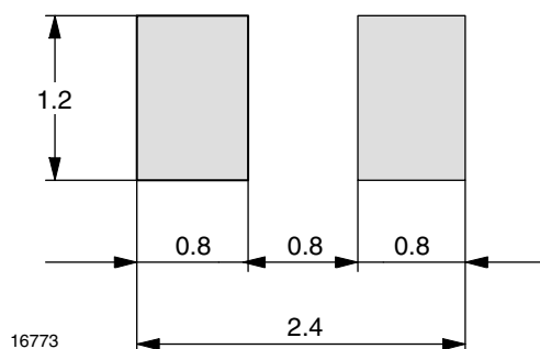
Fig. 11 - Recommended Foot Pads (in mm)
