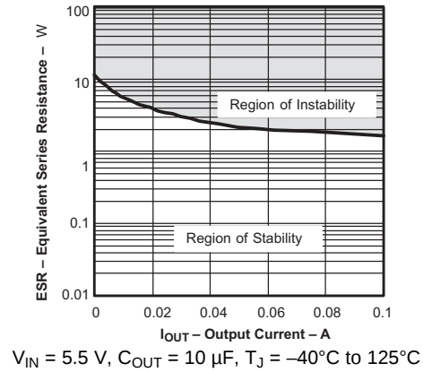
Figure 31. TPS79118 Typical Regions of Stability Equivalent Series Resistance (ESR) vs Output Current
