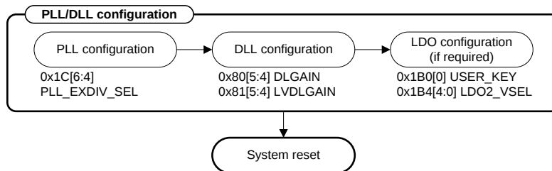
Figure 39 PLL/DLL Configuration
