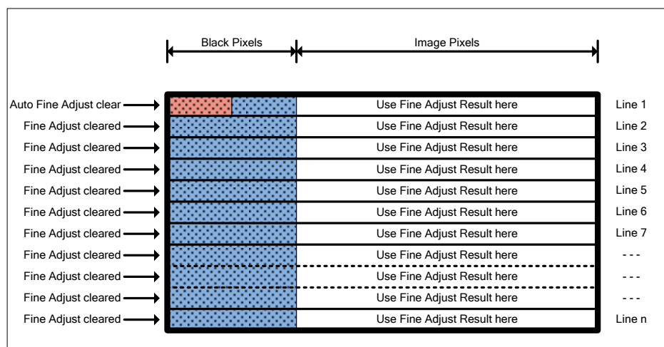
Figure 29 Scenario 1
