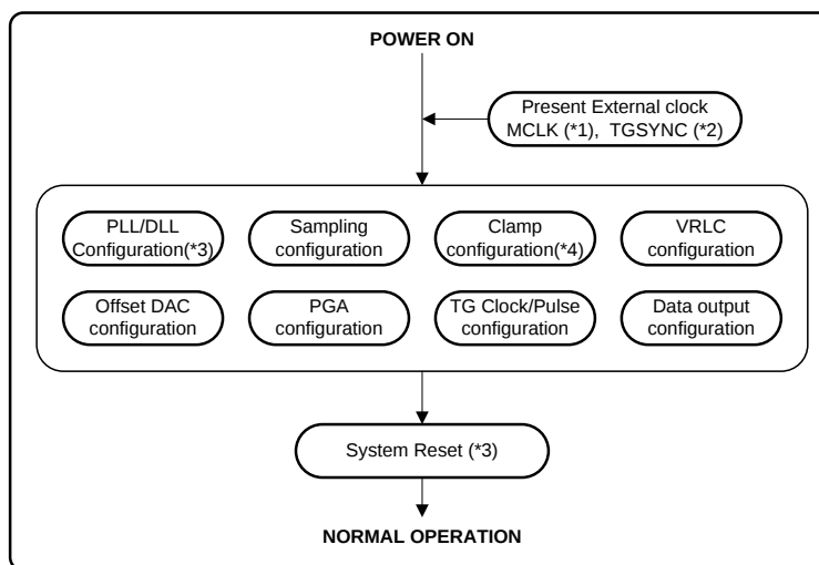
Figure 38 Overall Procedure
