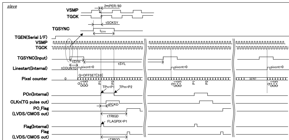
Figure 23 Slave Mode Pixel Counter and Line Start Timing
