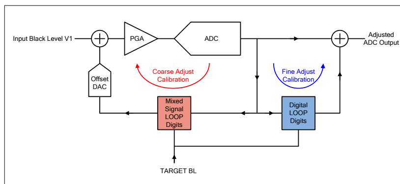
Figure 28 BLC Top-Level Circuitry
