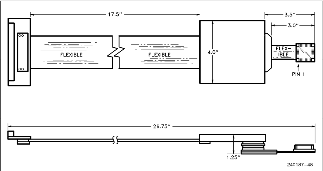
Figure 7.12. Preliminary ICETM-Intel386TM SX Emulator User Cable with PQFP Adapter
