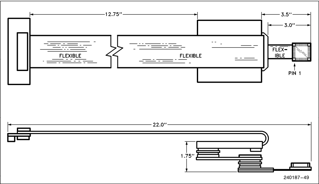
Figure 7.13. Preliminary ICETM-Intel386TM SX Emulator User Cable with OIB and PQFP Adapter
