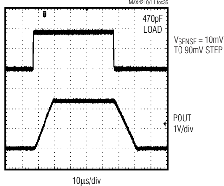
IOUT LARGE-SIGNAL PULSE RESPONSE
