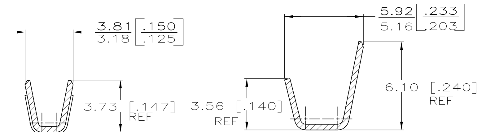
SECTION B-B
