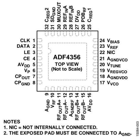
Figure 3. Pin Configuration
