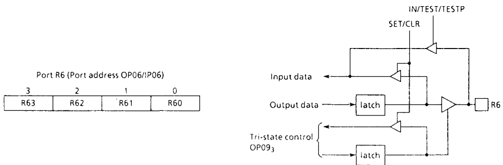
Figure 2-2. Port R6
