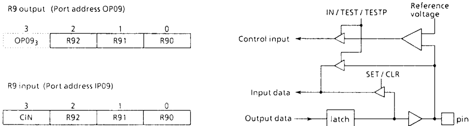
Figure 2-3. Port R9
