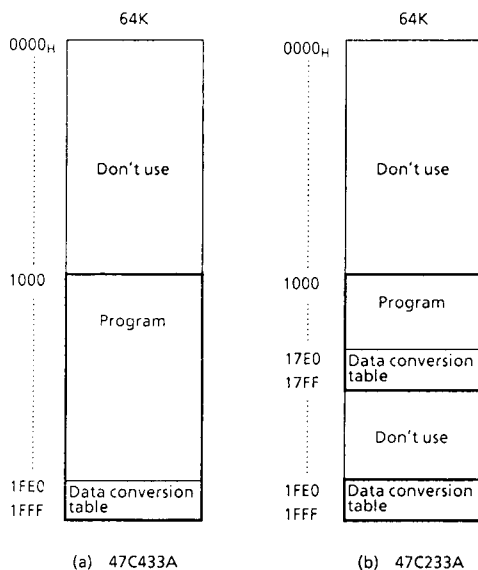
Figure 1. Program area
