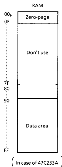
Figure 2. RAM addressing
