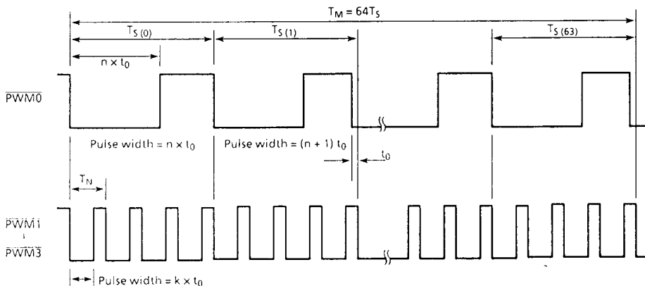
Figure2-6. \overline{\text{PWM}} Output Waveform (It is shown to the additional pulse T_S(1) and T_S(63) of the \overline{\text{PWM0}} )
