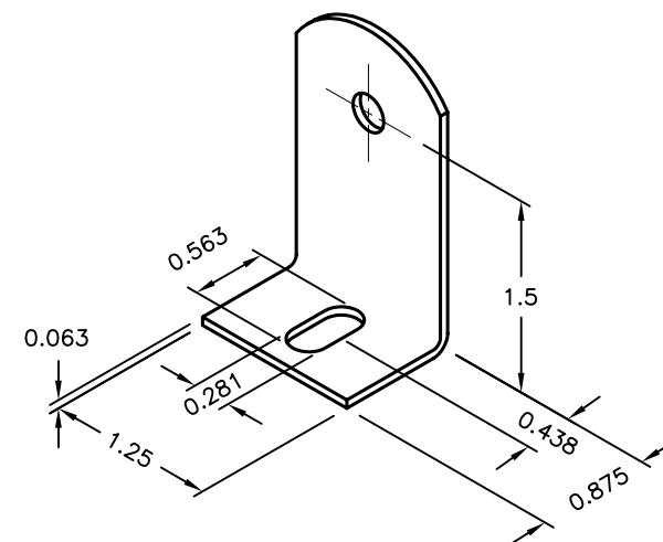
Brackets Dimensions
