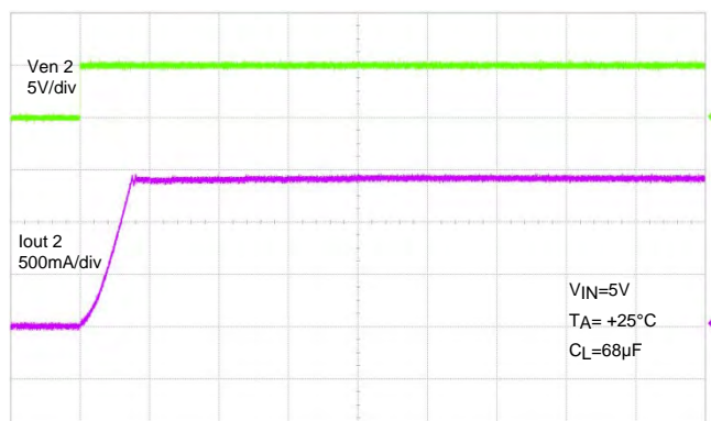
500µs/div Channel 2 Short Circuit Current, Device Enabled Into Short
