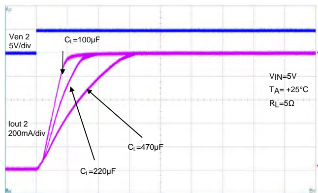
1ms/div Channel 2 Inrush Current
