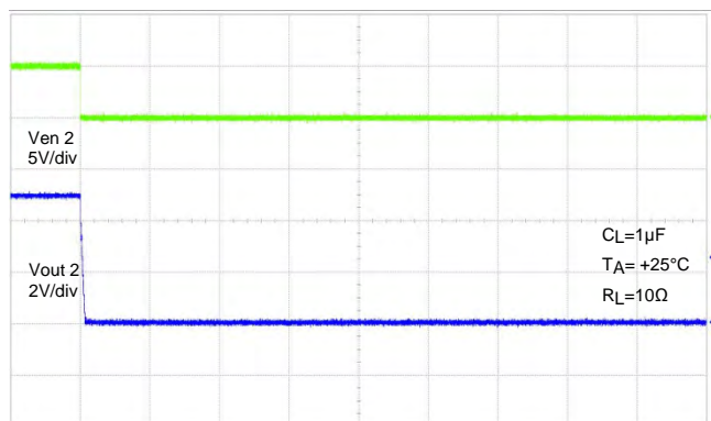
500µs/div Channel 2 Turn-Off Delay and Fall Time
