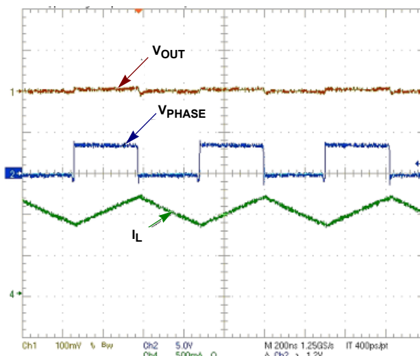
FIGURE 8. STEADY-STATE ( V_{IN} = 3.6V ; V_O = 1.6V ; I_O = 1A )
