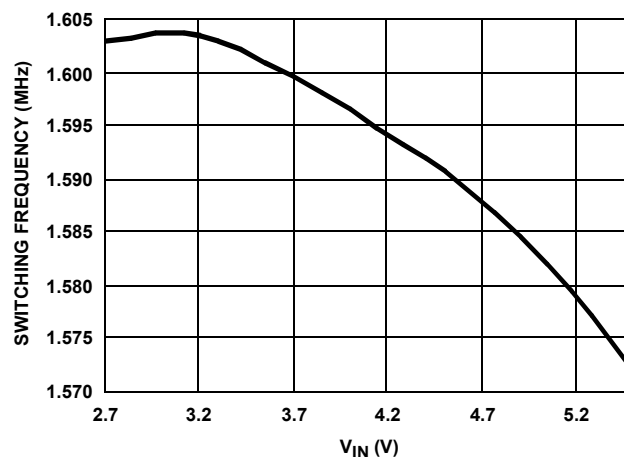
FIGURE 4. SWITCHING FREQUENCY vs V_{IN}
