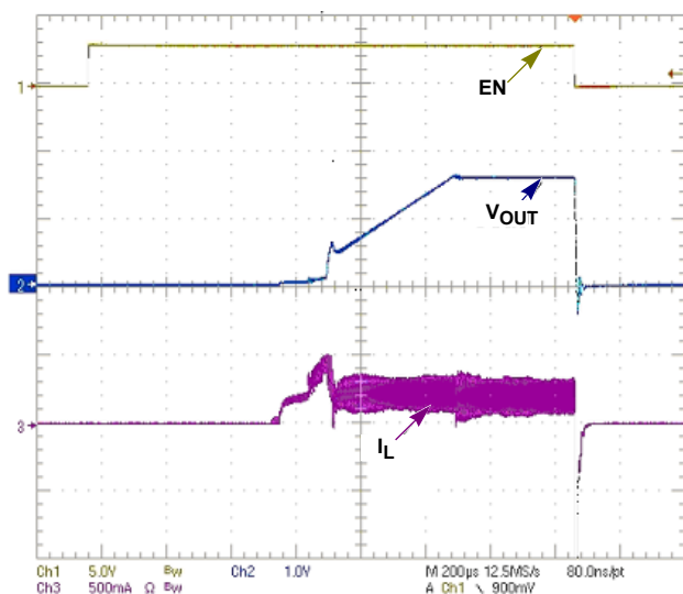
FIGURE 7. SOFT-START
