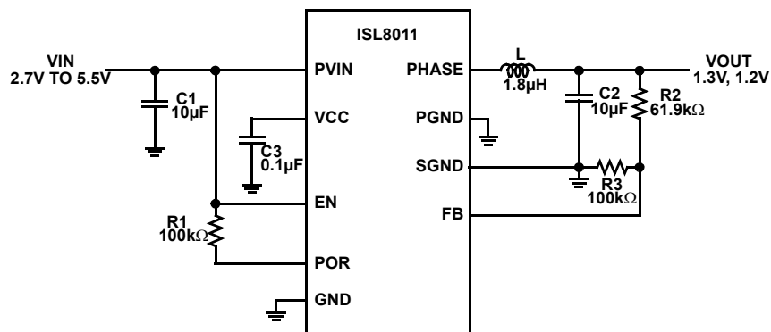
FIGURE 10. TYPICAL APPLICATION FOR ADJUSTABLE VERSION
