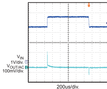
Line Transient with Resistive Load V_{IN}=3.5V-4.5V , V_{OUT}=2.50V , C_1=0 , I_{OUT}=250mA
