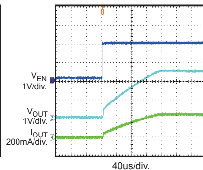
EN Start Up with Resistive Load I_{OUT}=250mA
