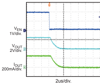
EN Shut Down with Resistive Load I_{OUT}=250mA
