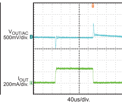
Load Transient with Resistive Load I_{OUT}=10mA-250mA
