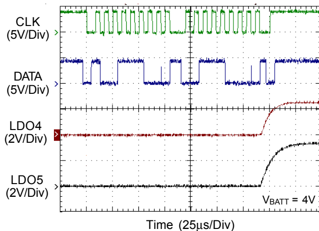
I 2 C Power On LDO4, LDO5
