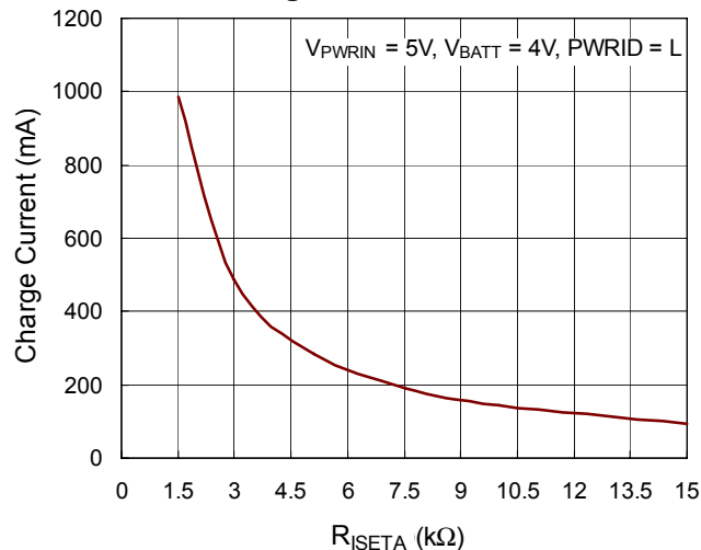
Charge Current vs. RISETA
