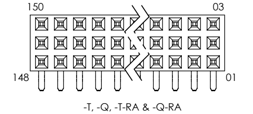
FIG 3 POLARIZATION LOCATION (INSERT PK-06-N INTO SPECIFIED POSITION & BREAK OFF TAB) (-RA OPTION SHOWN FOR ORIENTATION PURPOSE ONLY)
