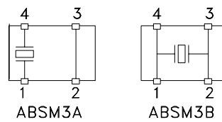
Electrode arrangement
