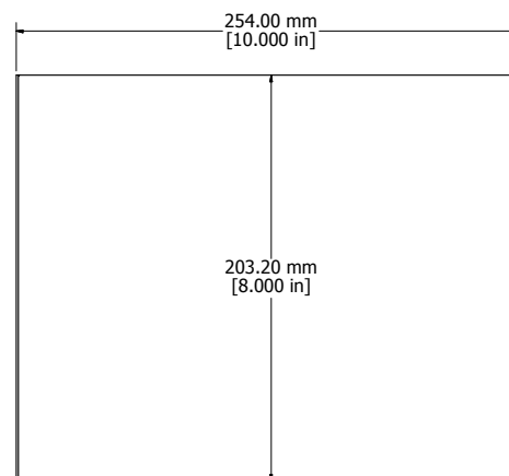
BOTTOM/TOP ENCLOSURE
