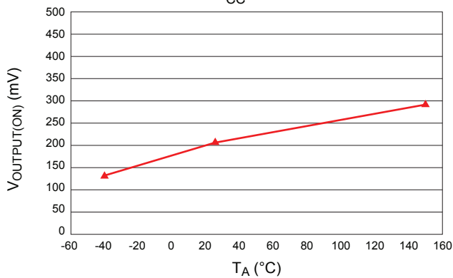
Low Output Voltage versus Ambient Temperature V_{CC} = 12\text{ V}
