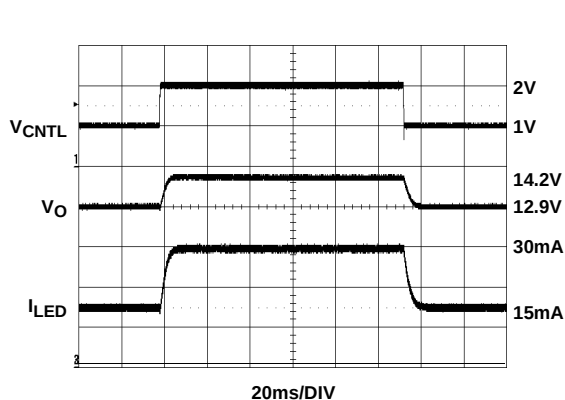
FIGURE 16. TRANSIENT RESPONSE
