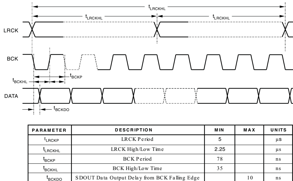
Figure 6. Master and Slave Mode Audio Serial Port Timing: Left Justified, Right Justified, and Philips I 2 S
