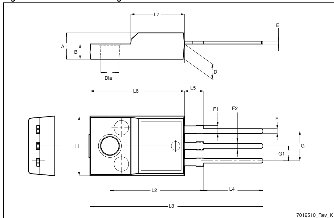
Figure 23. TO-220FP drawing
