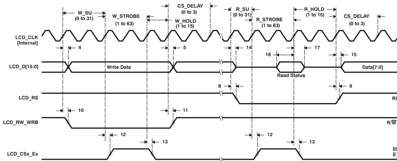
Figure 5-30. Character Display HD44780 Write
