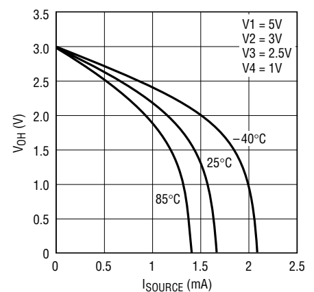
RST High Level Output Voltage vs Output Source Current (LTC2902-2)
