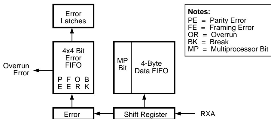
Figure 31. ASCII Receiver
