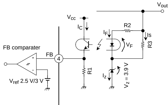
Figure 2 Ripple Voltage Establish (example)
