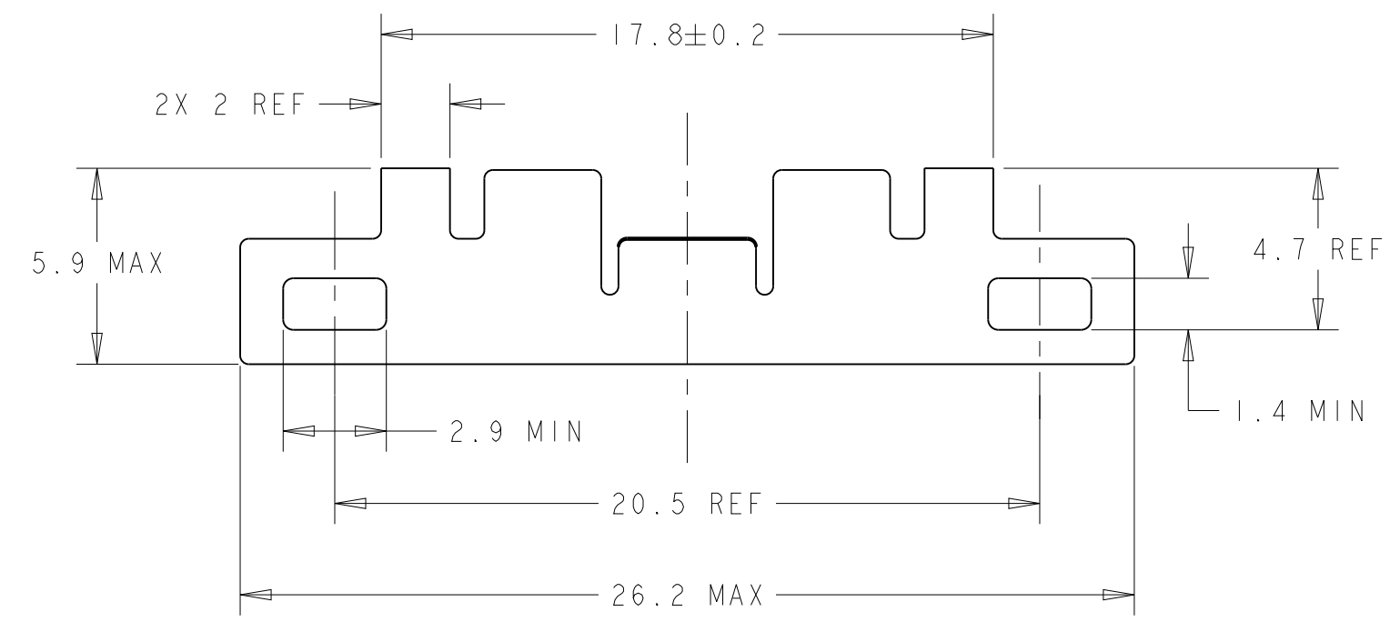
2007304-1 AS SHOWN SCALE 5:1
