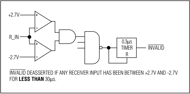
Figure 2b. INVALID Functional Diagram, INVALID High
