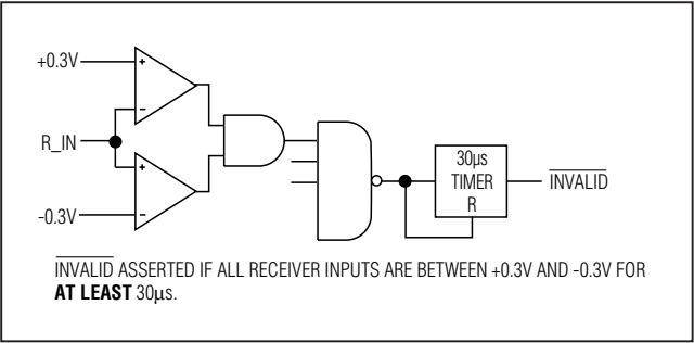
Figure 2a. INVALID Functional Diagram, INVALID Low
