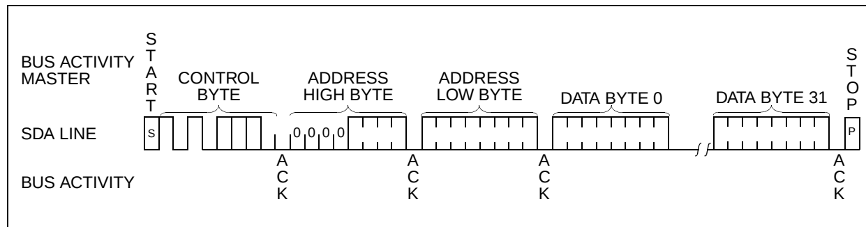
FIGURE 4-2: PAGE WRITE
