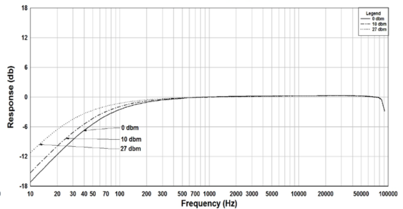
109R Rs=10K, RI=1500 Frequency Response
