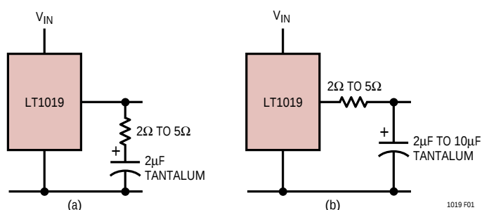
Figure 1. Output Bypassing
