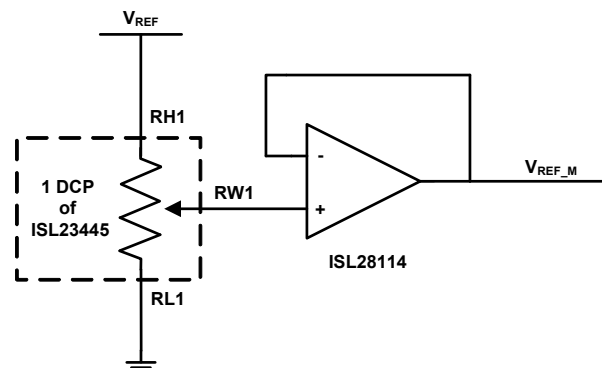
FIGURE 2. V_{\text{REF}} ADJUSTMENT
