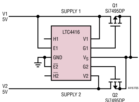
Figure 5. Dual PowerPath for Current Sharing
