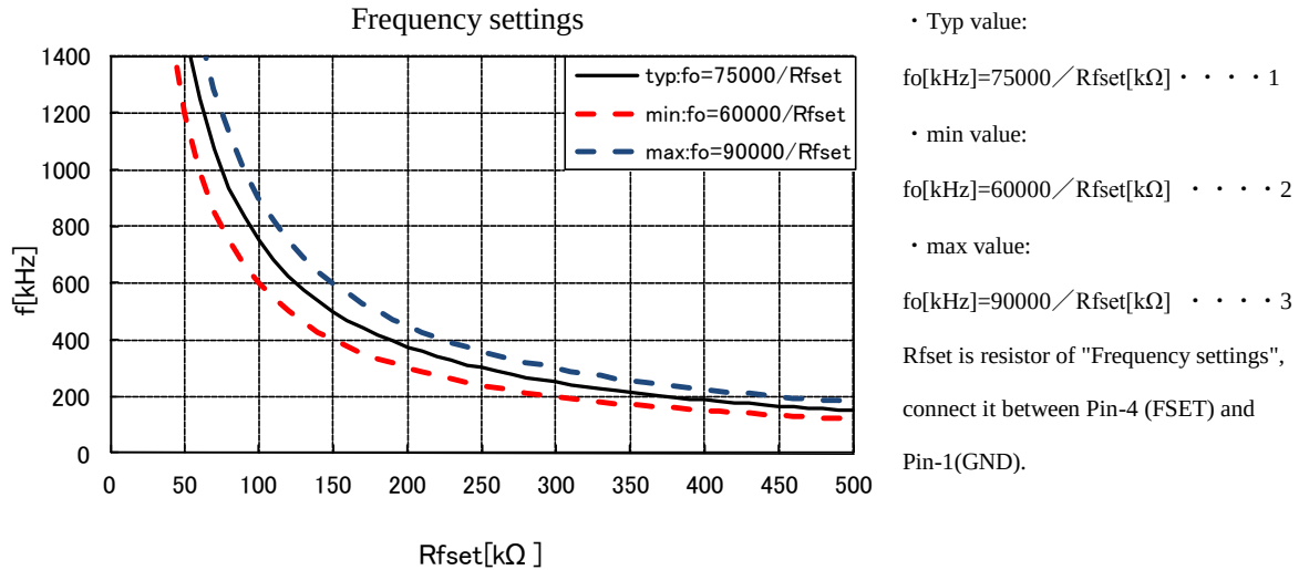
Fig. 24 Characteristic of Operational Frequency
