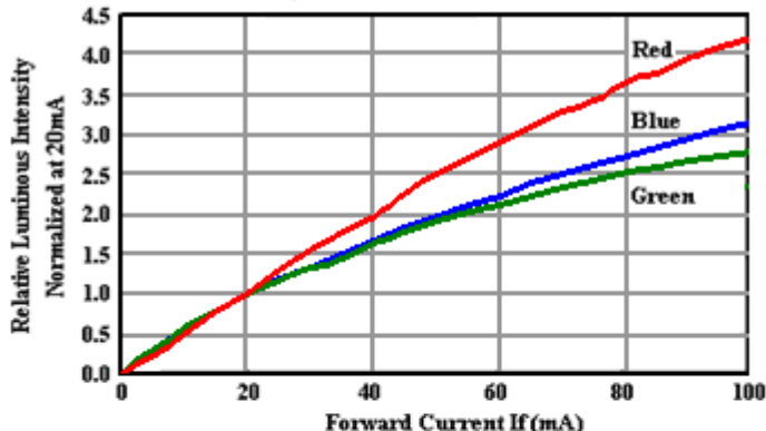
Fig.4 Relative Luminous Intensity vs Forward Current
