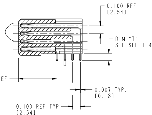
SECTION X-X
