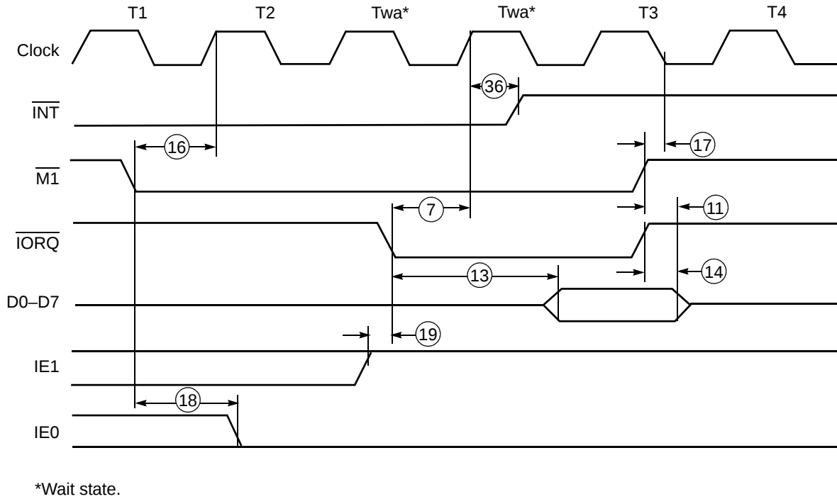
Figure 35. Interrupt Acknowledge Cycle
