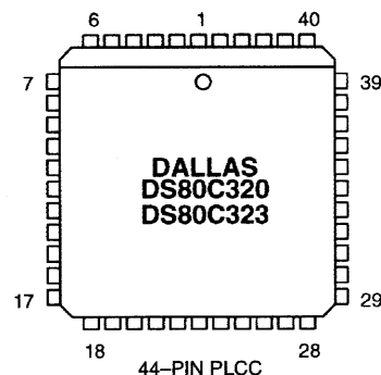
44-PIN PLCC
