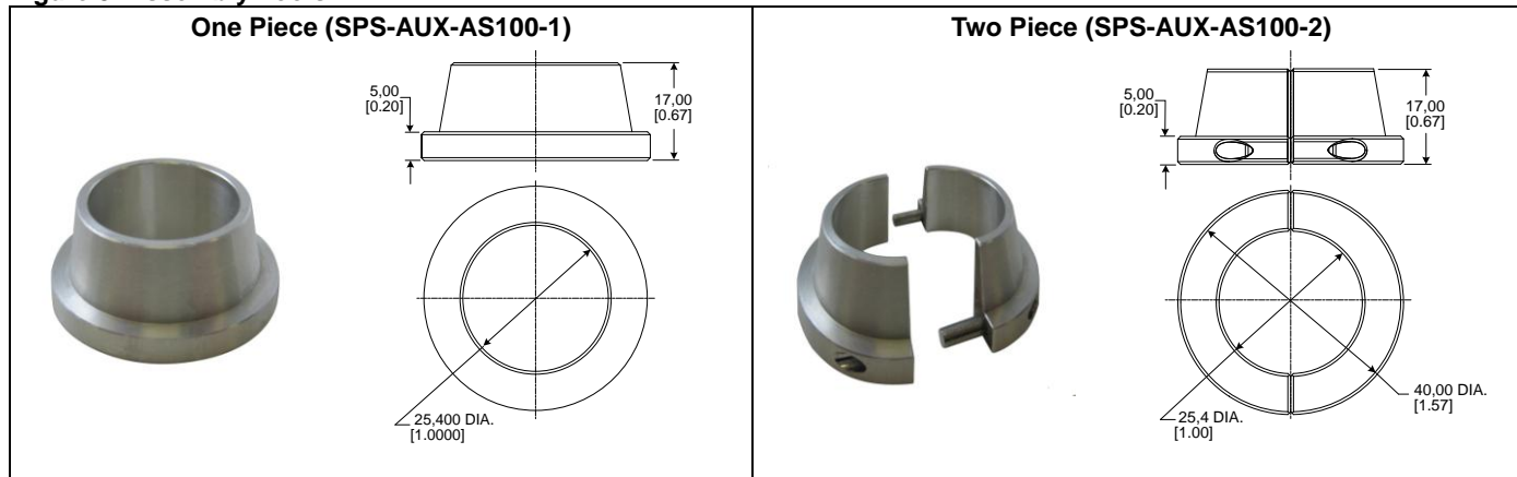
Figure 3. Assembly Tools
