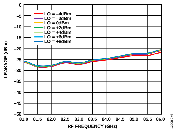
Figure 45. 6x LO Leakage at RFOUT vs. RF Frequency at Various LO Powers, I_{FIN} = 5 dBm, IF = 1000 MHz, USB
