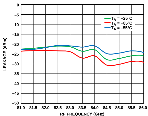
Figure 53. 6x LO Leakage at RFOUT vs. RF Frequency at Various Temperatures, IFIN = 5 dBm, IF = 500 MHz, LSB
