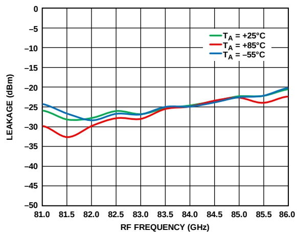
Figure 42. 6x LO Leakage at RFOUT vs. RF Frequency at Various Temperatures, I_{FIN} = 5 dBm, LO = 2 dBm, IF = 2000 MHz, USB
