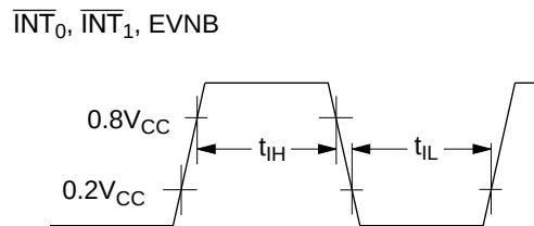
Figure 57 Interrupt Timing
