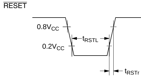
Figure 58 \overline{RESET} Timing
