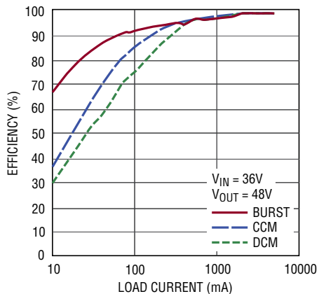
Efficiency vs Output Current (Boost Region-Figure 14)
