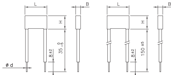
Insulated rigid leads
