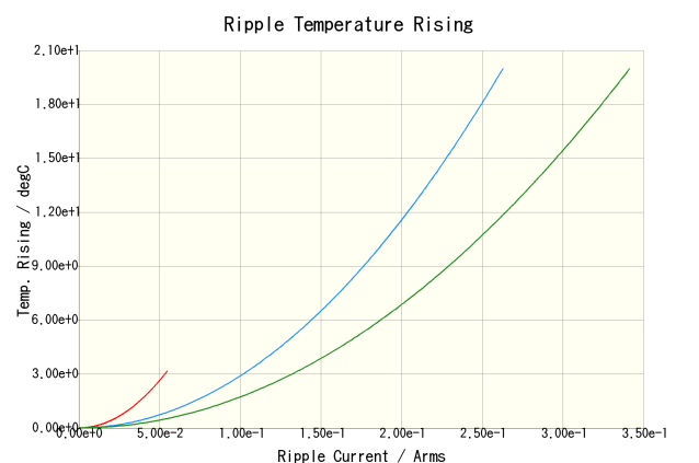
C1608X7R1E103K080AA(100kHz) C1608X7R1E103K080AA(500kHz) C1608X7R1E103K080AA(1MHz)
