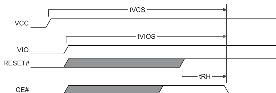
Figure 10.3 Power-Up Diagram
