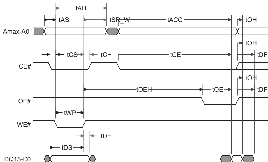
Figure 10.10 Write to Read ( t_{CE} ) Operation Timing Diagram
