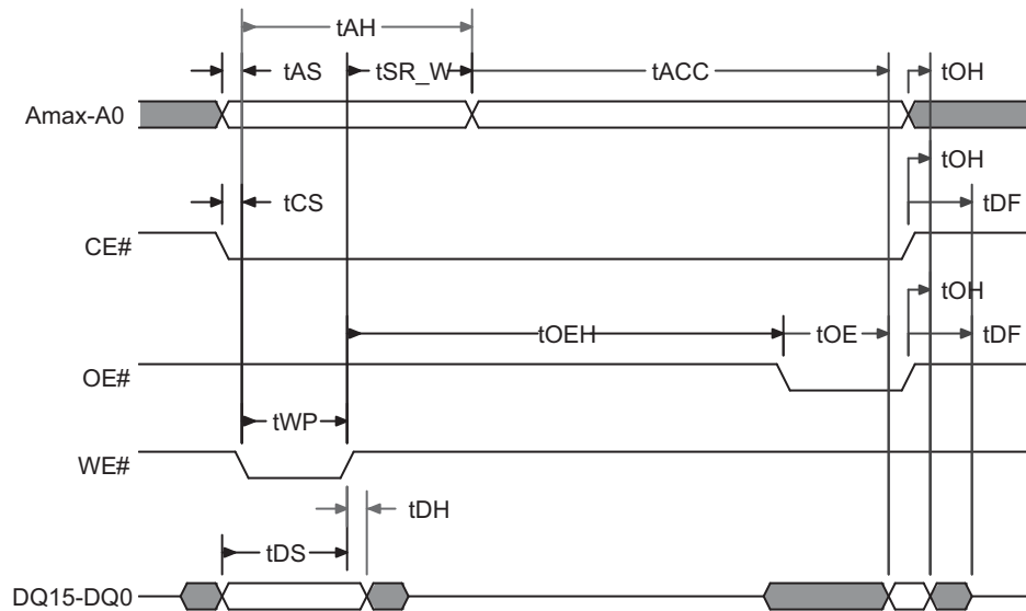
Figure 10.9 Write to Read ( t_{ACC} ) Operation Timing Diagram
