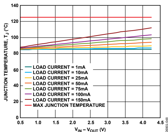
Figure 46. TSOT, 100\text{ mm}^2 of PCB Copper, T_A = 85^{\circ}\text{C}
