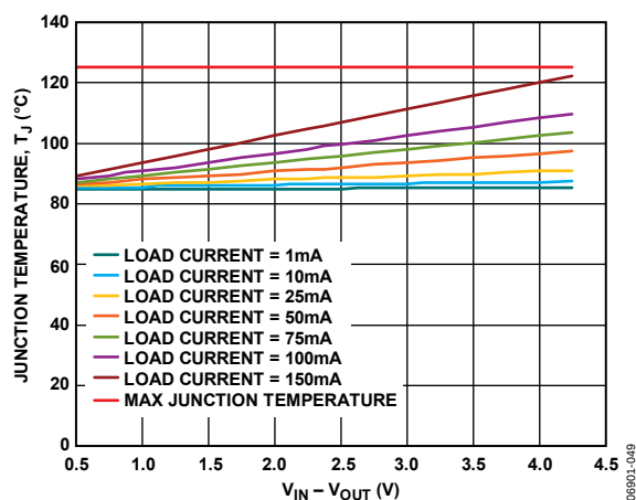
Figure 47. WLCSP, 100\text{ mm}^2 of PCB Copper, T_A = 85^{\circ}\text{C}
