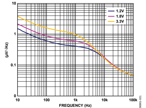
Figure 21. Output Noise Spectrum, V_{IN} = 5\text{ V} , I_{LOAD} = 10\text{ mA} , C_{OUT} = 1\text{ }\mu\text{F}
